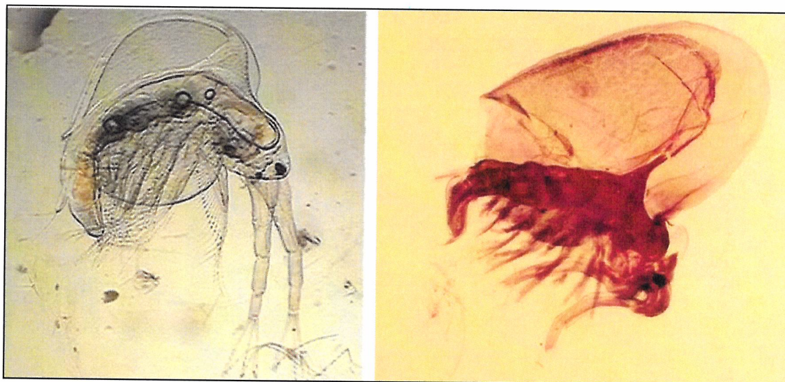
Fig. 4.2 Two pictures of Holopedium gibberum , a cladoceran zooplankton that dominated the zooplankton community of all of the lakes surveyed.
